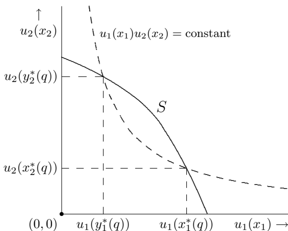
Figure 4.2 An illustration of the proof of Proposition 4.2.
